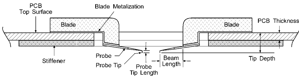
Figure 3. Blade probe card with blades attached.
