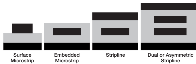
Figure 16. Signal layout for controlled impedance. Blue areas represent dielectric material; black represents ground or signal traces.
