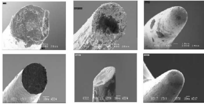
Figure 28. Before and after a non-abrasive clean.
