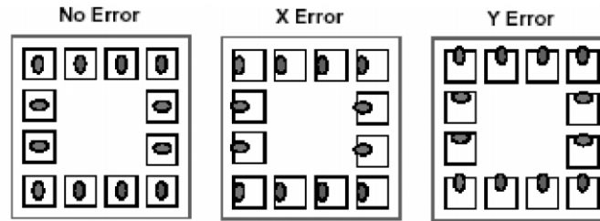
Figure 23. Probe alignment examples.
