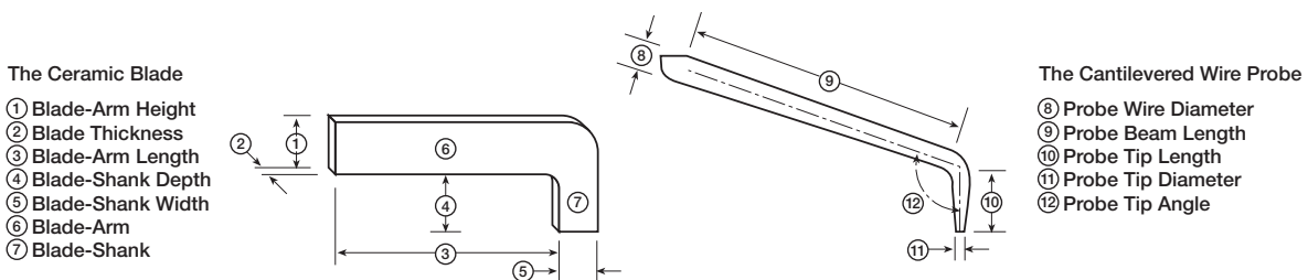
Figure 8. Ceramic blade probe geometries.
