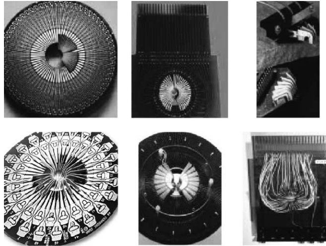
Figure 5. Different types of ceramic blade probe cards.
