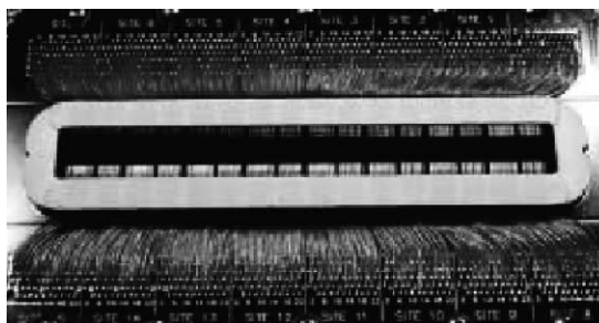
Figure 1. Multi-DUT memory probe card.
