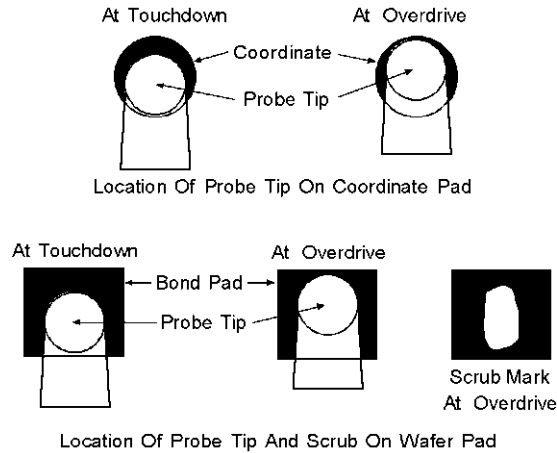
Figure 21. Location of probe tip and scrub on wafer pad.
