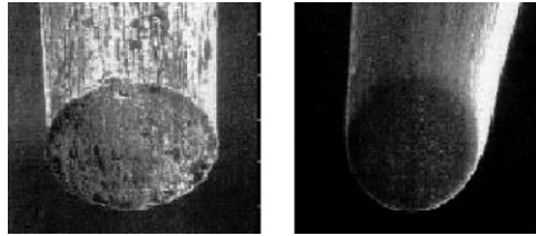
Figure 18. Flat and semi-radius tip shapes.
