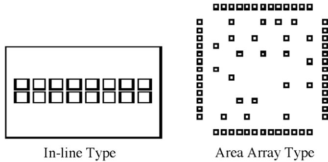
Figure 10. Bond pad configuration types.
