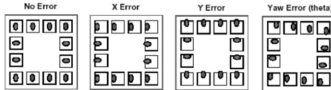
Figure 24. Scrub mark definition.
