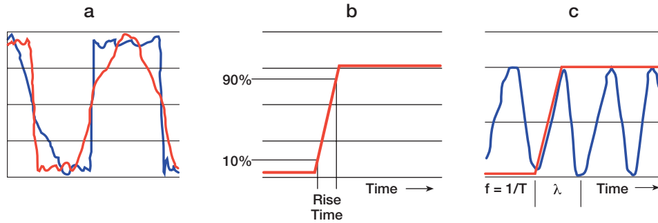
Figure 29. Square wave harmonics.
