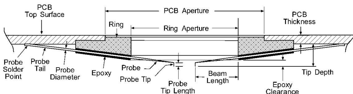
Figure 2. Epoxy card with ring assembly.
