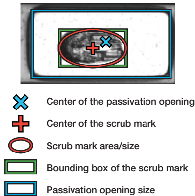
Figure 25. Five scrub mark characteristics.
